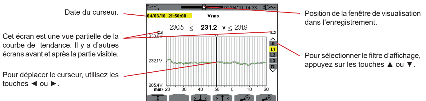
Figure 95 : Vrms (L1) sans MIN-AVG-MAX
