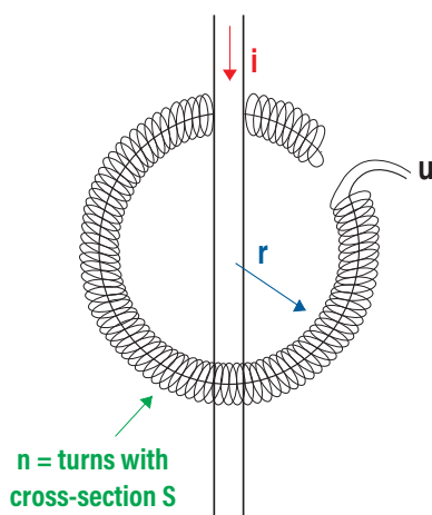
• Rogowski coil
