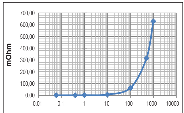
Insertion impedance
